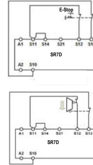
Fig. 7: Dual channel emergency stop with ground fault monitoring. (Category 3, up to PL d / SIL 2)
